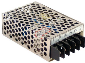
Nätaggregat Mean Well RS-15-48, 48 VDC (43.2...52.8) 15W
