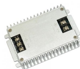
DC/DC- Boost Buck Converter, stabilisator 12VDC (8...36VDC) till
