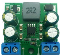
DC-DC Step-Up Boost Converter Module, 12V 3A
