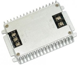
DC/DC- Isolated Buck Converter, 36-75VDC till 5VDC 20A
