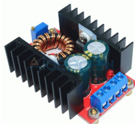
DC-DC Boost Converter Step Up Power Supply Module 10-32V Till 35-60V,
