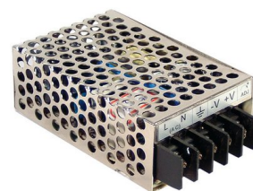
Nättaggregat Mean Well RS-25-3, 3.3 VDC (2.9...3.6) 25W
