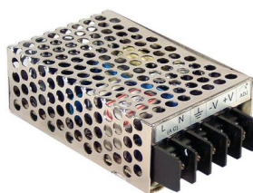
Nättaggregat Mean Well RS-35-3, 3 3 VDC (2.9...3.6) 35 W
