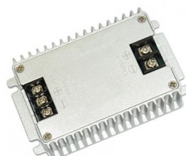
DC/DC- Isolated Buck omvandlare, 36-75VDC till 12VDC 10A
