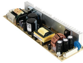
Switchat nättaggregat Mean Well LPS-100-7.5 13.3A
